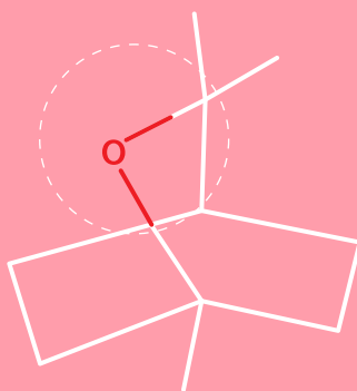
Figure 13: An example of an ether group in the compound eucalyptol, the main constituent of Eucalyptus oil
